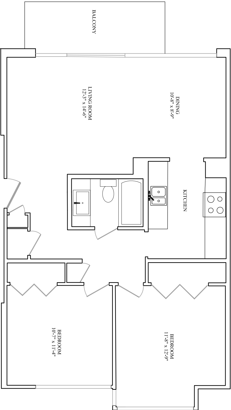
BERN STREET - FLOOR PLAN A TWO BEDROOM 2ND FLOOR - BALCONY / GROUND FLOOR - PATIO
